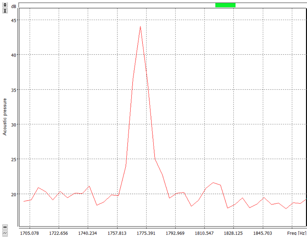
Figure 5.1 FFT analysis (Location 1)
