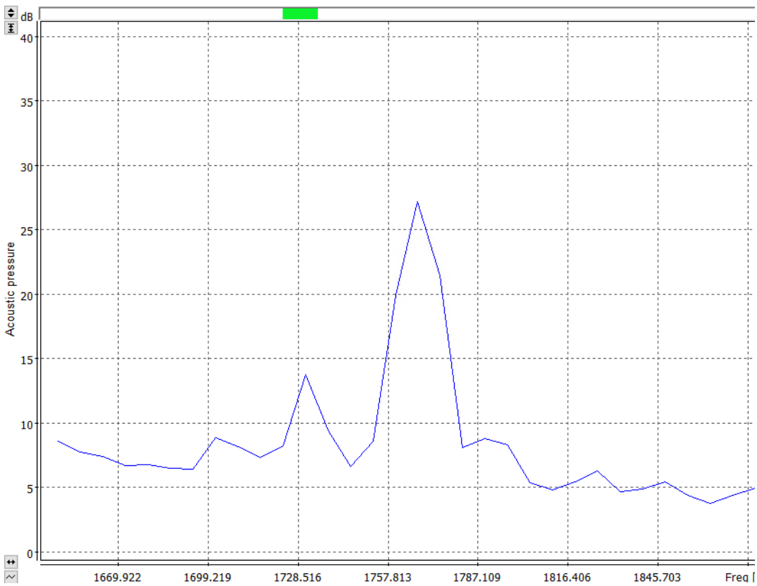
Figure 5.2 FFT analysis (Location 2)
